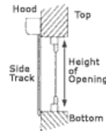
Example of Surface Mount Installation Drawing 2
